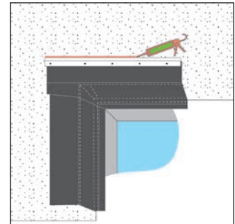
Fig 2: Final Stage – Clamping strip sealing with OT015 Paste Adhesive
